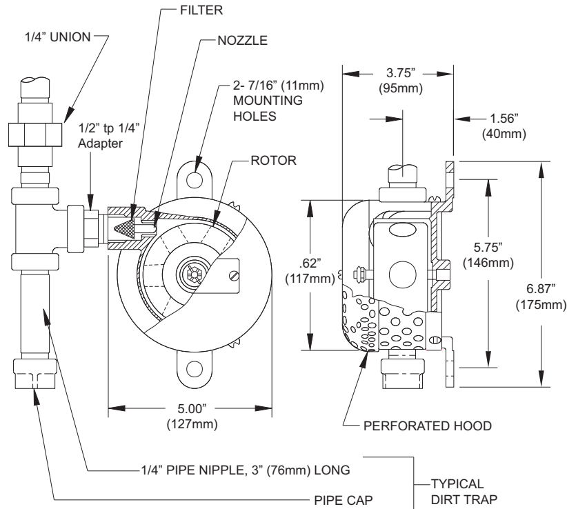
Figure 1. Nitrogen Pressure Operated Siren
